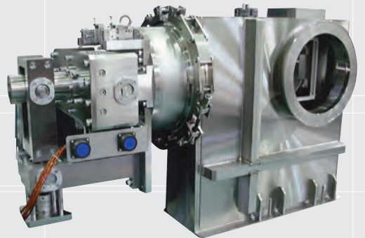
■ Proton Beam Profile Monitor (variable drive type)
